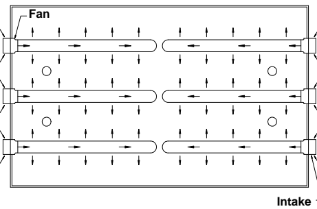
Sidewall Mount Plan View
